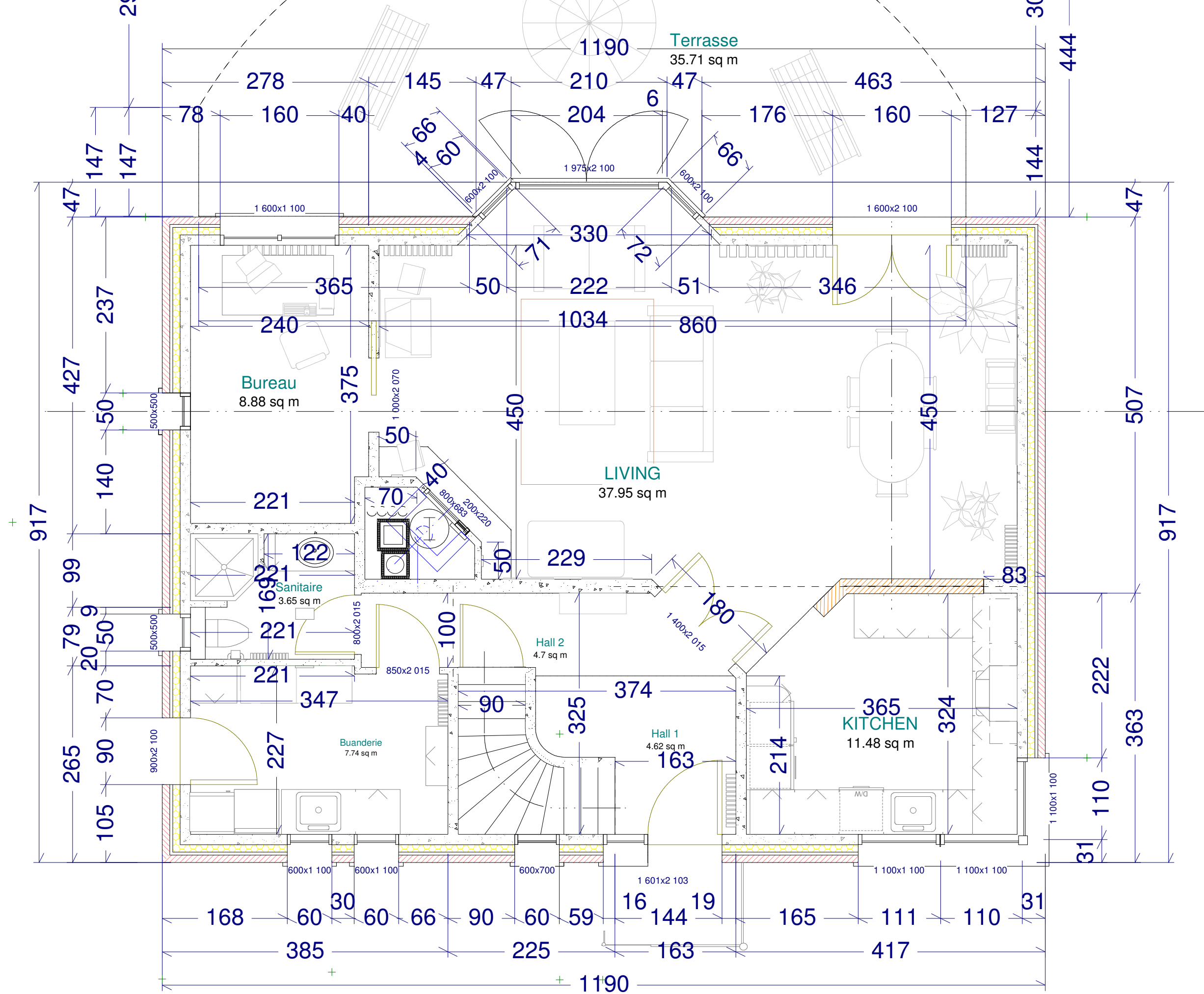
LIVING AREA 92. sq m
